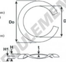
Split Wave Spring Washers
