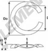
Split Wave Spring Washers
