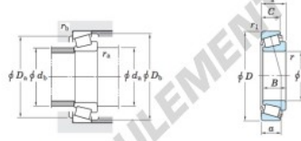
Single-row tapered roller bearings inch series
