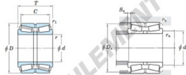
Double-row tapered roller bearings TDO type Koyo
