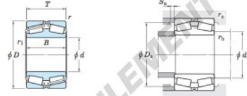
Double-row tapered roller bearings TDI type Koyo
