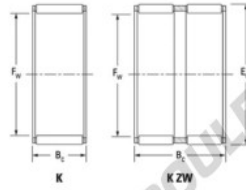
Radial needle roller and cage assemblies
